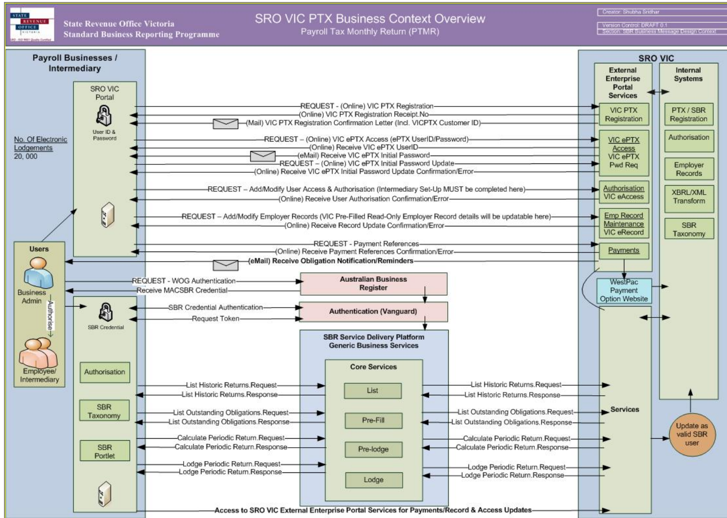
Figure 1 – SRO VIC Payroll Tax Business Context Overview
