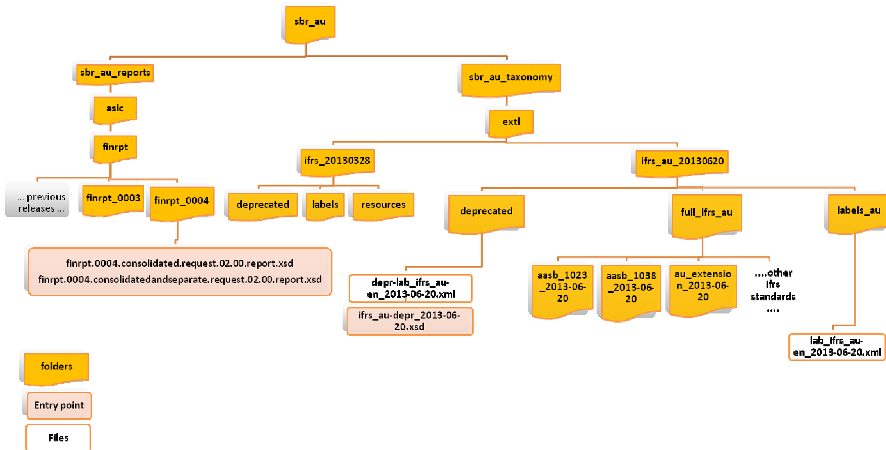
Illustration 5 Folders and files structure
