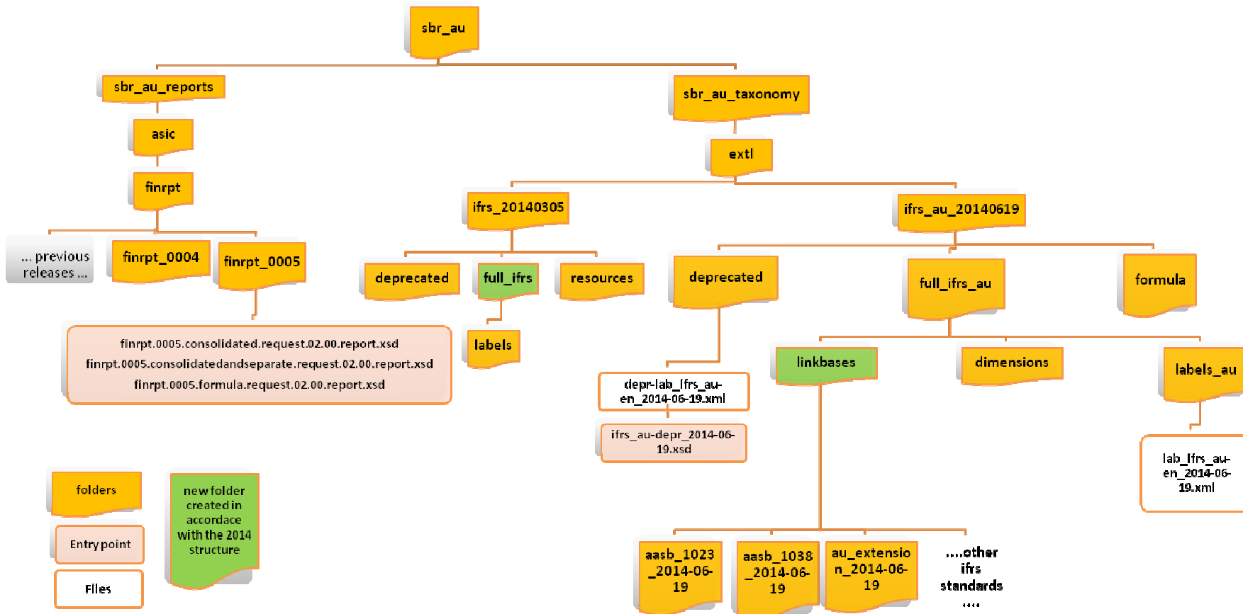
Illustration 5 Folders and files structure
